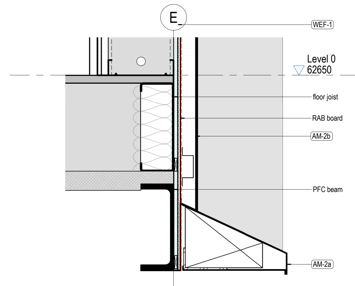
10 Base Level Flashing Detail 1:5 Typical
