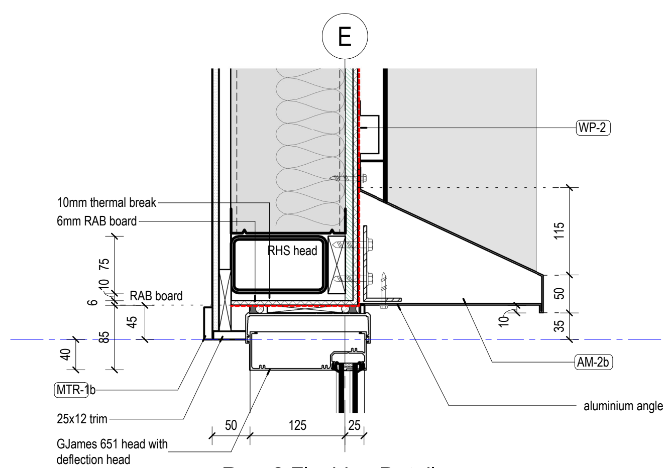
7 Row 2 Flashing Detail 1:5 Typ. Window Head
